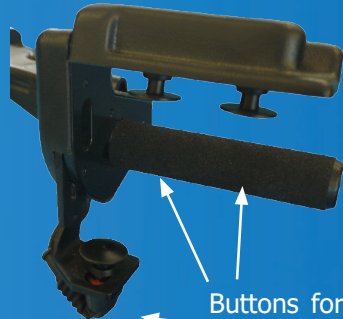
CL002A Handle (push = brake / pull = accelerator)
